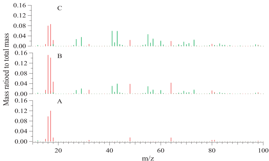
Fig. 4. AMS MS traces of ammonium sulfate/palmitic acid aerosol. The green indicate organic peaks and the red are sulfate peaks, A) pure ammonium sulfate; B) bath set to 120^{\circ}\text{C} (internally mixed aerosols that are 48.8 wt% organic/51.2 wt% ammonium sulfate); and C) bath set to 140^{\circ}\text{C} (partially externally mixed aerosols that have an overall composition of 81 wt% organic/19 wt% ammonium sulfate).
